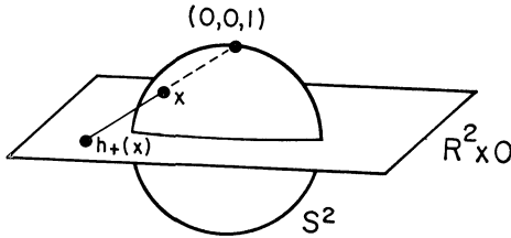
Figure 3. Stereographic projection
